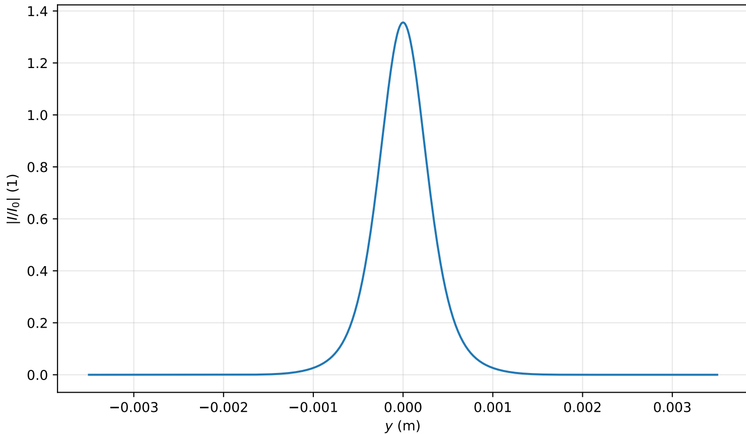
Intensity profile I(x=0, y, z=1.433)/I_0 , P_{in}=0.8P_{cr} , artificial time
